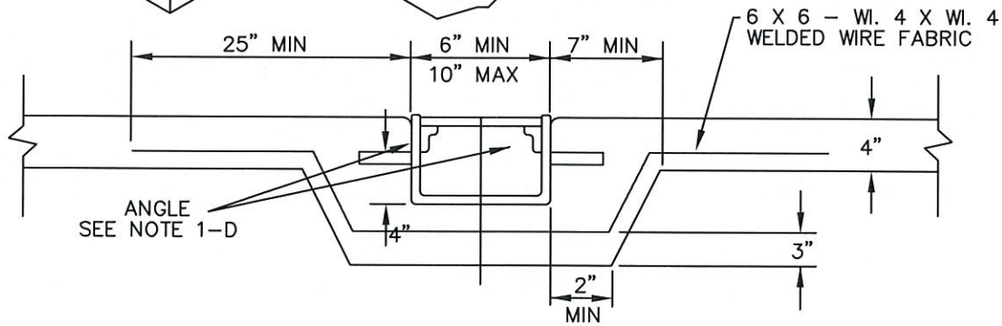
SECTION B-B END VIEW
