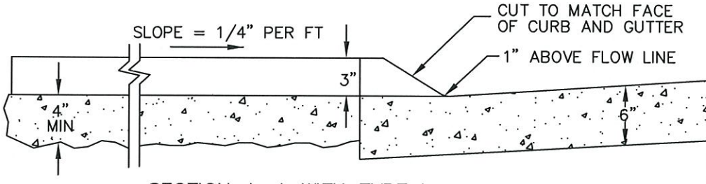
SECTION A-A WITH TYPE I CURB AND GUTTER
