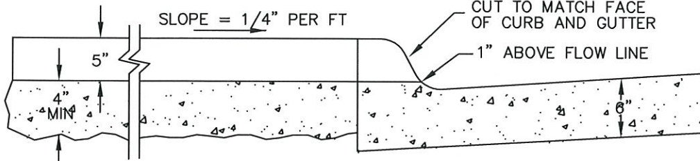
SECTION A-A WITH TYPE II CURB AND GUTTER
